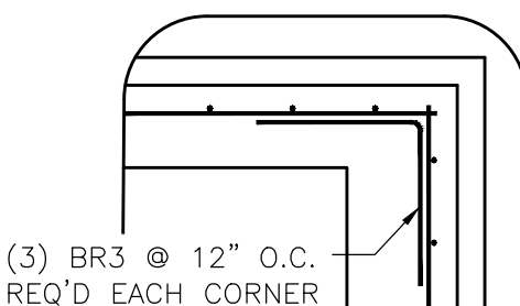
CORNER REINFORCING DETAIL
