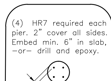
SAFETY PIER REINFORCING Top View
